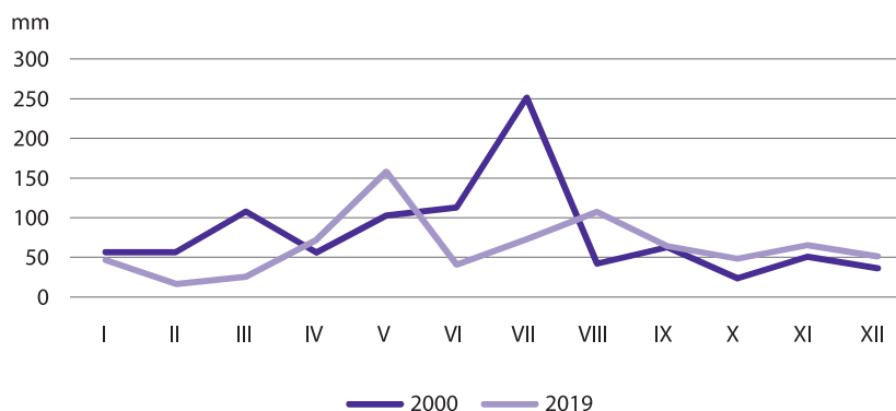
Chart 7. Average monthly total atmospheric precipitation
