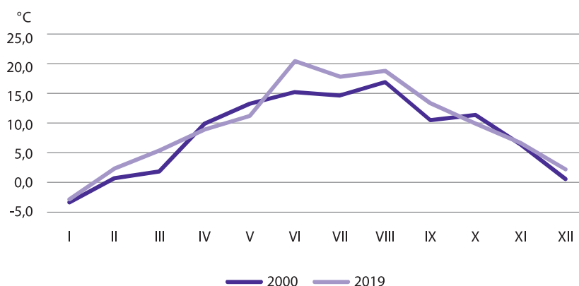
Chart 6. Average monthly air temperature
